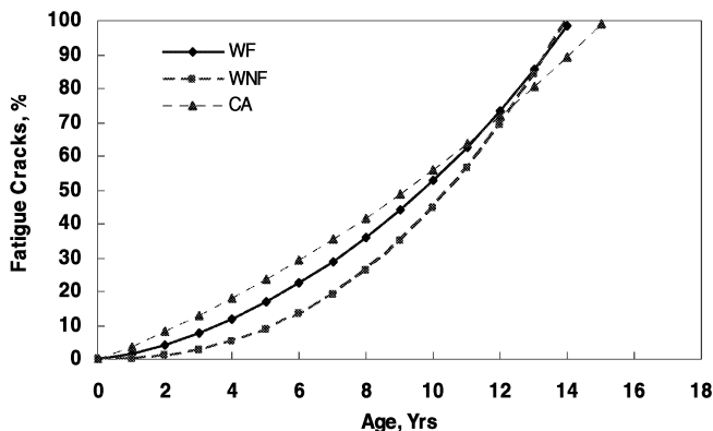
Fig. 11. Variation of Fatigue Cracks with Age.
