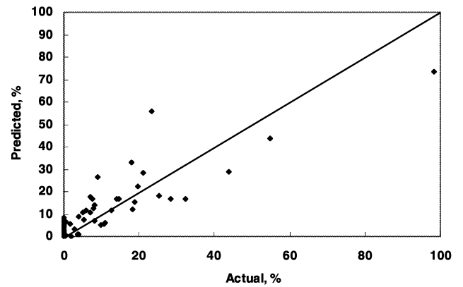
Fig. 8. Actual vs. Predicted Fatigue Cracks Percentage for the WF Region Model.
