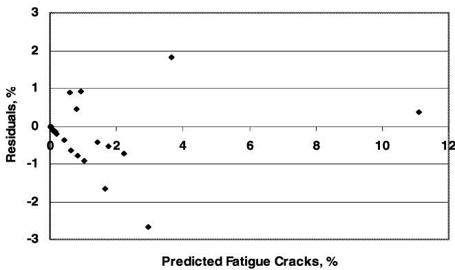
Fig. 6. Residuals vs. Predicted Fatigue Cracks for the WNF Region Model.
