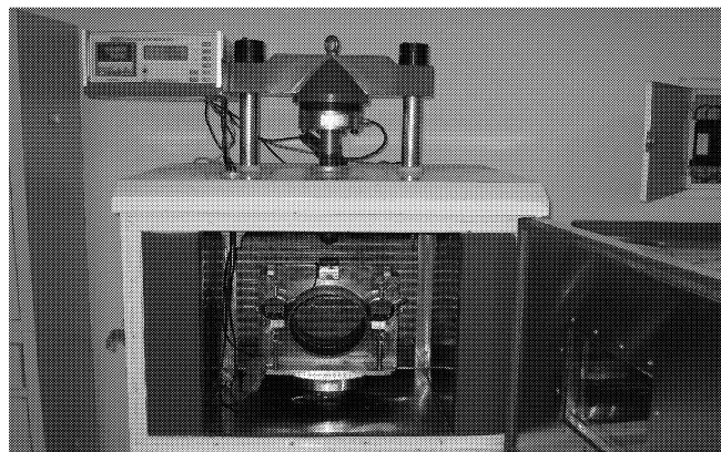
Fig. 4. Loading Equipment Equipped with Shear Device.
