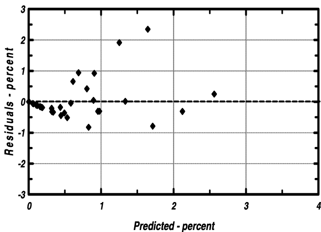
Fig. 6. Predicted versus Residuals for the WNF Region Model.
