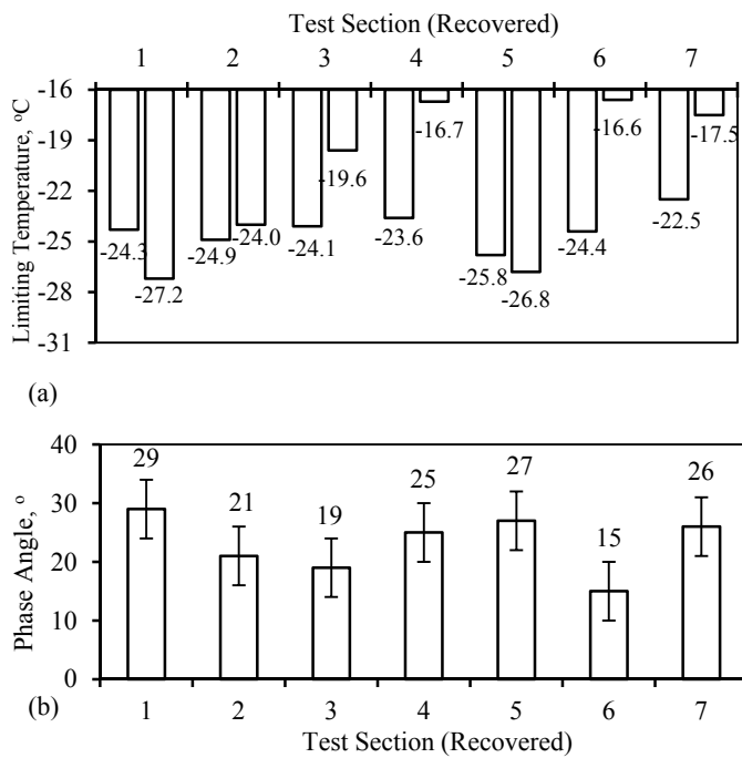
Fig. 6. Conventional grading of asphalt cements recovered from 2009 core samples: (a) BBR and (b) DSR at -14°C. Note: Limiting stiffness temperatures are provided in the first column and limiting m-value temperatures in the second column. Error bars on phase angles provide ± 1 pooled standard deviation. Significant errors in DSR data show that at this temperature the machine is at the limit of its capabilities with 8 mm parallel plates.
