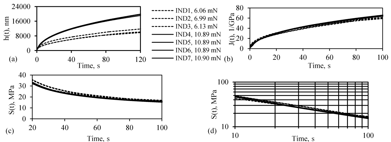
Fig. 2. Typical indentation creep results obtained from a 200 micron thin asphalt cement film at -14°C: (a) Raw data at different creep loads; (b) Compliance versus time at different creep loads; (c) Stiffness versus time at different creep loads; and (d) Creep stiffness master curve (i.e., log-log plot of Fig.2(c)).
