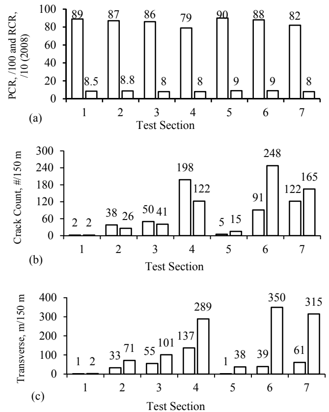
Fig. 7. Pavement distress indicators: (a) Pavement condition rating (PCR) and Ride comfort rating (RCR) indices for August 2008 [6]; (b) Approximate transverse crack counts for 2008 (first column) [6] and 2010 (second column); and (c) Approximate transverse crack lengths for 2008 (first column) [6] and 2010 (second column).
