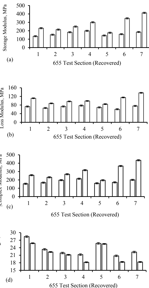
Fig. 5. Dynamic rheological data for recovered binders at 0.5 Hz and -8°C (first column) and -14°C (second column): (a) Storage moduli; (b) Loss moduli; (c) Complex moduli; and (d) Phase angles. Note: Error bars reflect \pm 1 pooled standard deviation.
