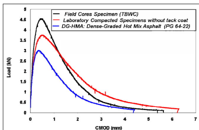
Fig. 7. Typical Load Crack Mouth Opening Displacement (CMOD) Plot.
