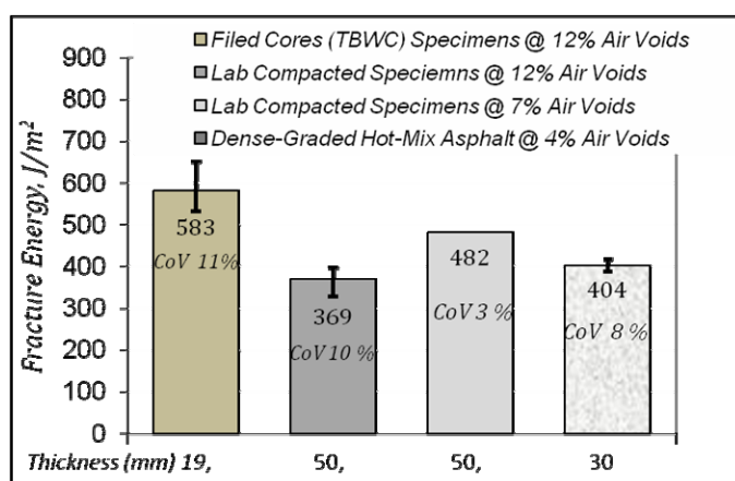
Fig. 12. Comparison of Fracture Energies of Different HMA Mixes.
