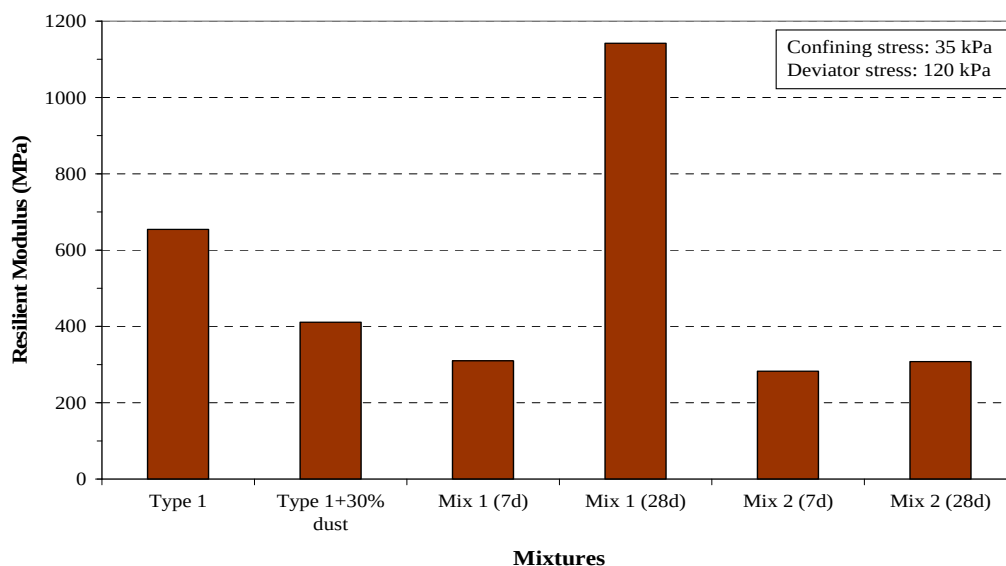
Fig. 3. 7 and 28 Day Resilient Moduli of Mix 1 and 2 in Comparison with Those of Ordinary and 30% Dust-Elevated Type 1.
