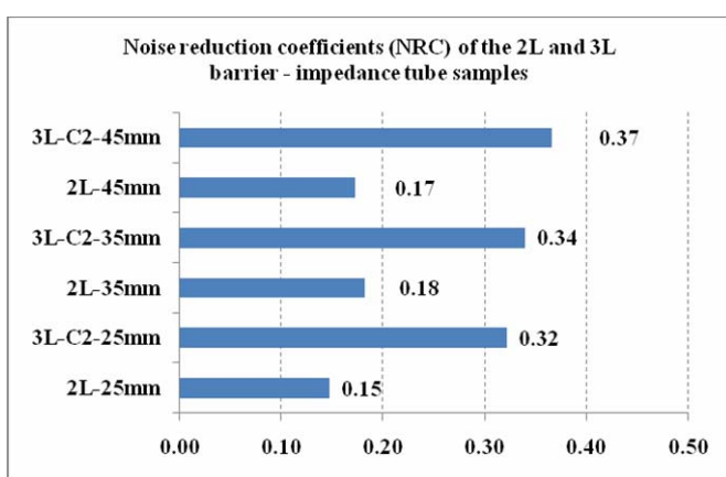
Fig. 8. NRC of Two and Three-Layered Samples Derived from Impedance Tube Testing.
