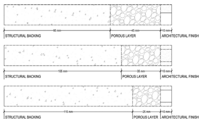
Fig. 2. Cross-Sections of Impedance Tube Samples.
