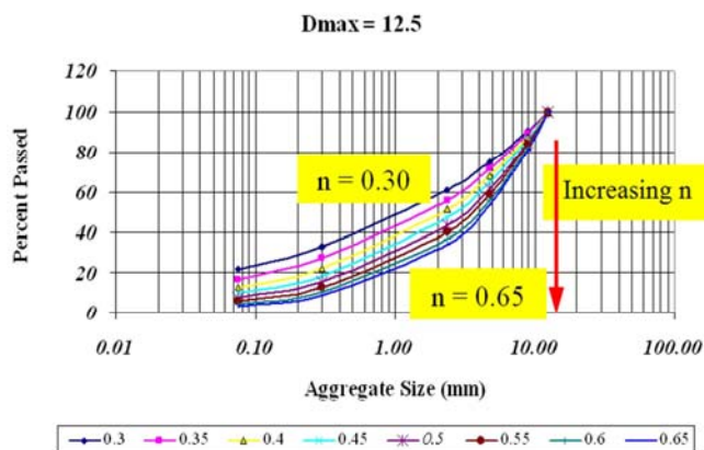
Fig. 2. Fuller Gradation Curves for Different Values of “n” and D_{\max} = 12.5\text{mm} .
