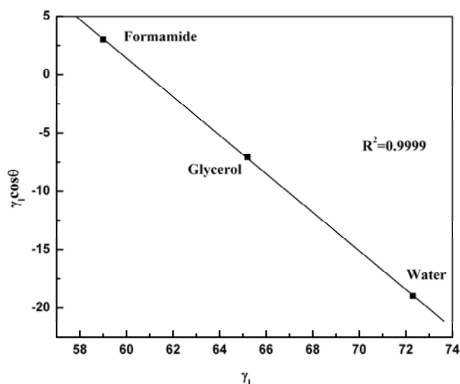
Fig. 4. Illustration of the \gamma_l \cos \theta versus \gamma_l for AAD-1 Asphalt Binder.
