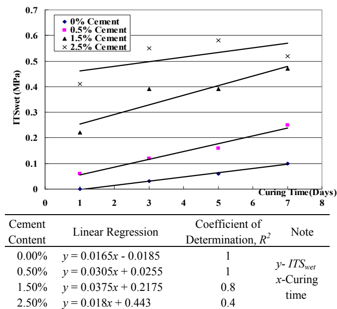
Fig. 5. Relationship between ITS_{wet} and Curing Time.
