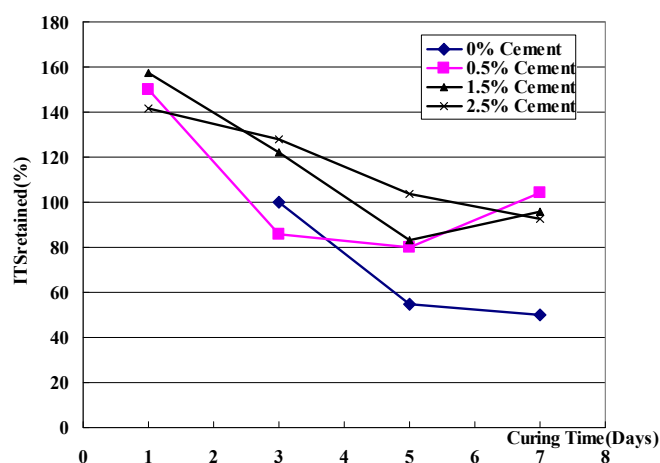
Fig. 8. Relationship Between ITS_{retained} and Cement Content.
