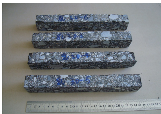
Fig. 2. Bending Beam Test Specimens.
