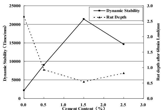
Fig. 10. Relationship Between DS and Cement Content.
