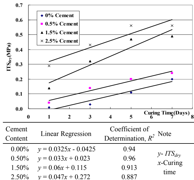
Fig. 4. Relationship between ITS_{dry} and Curing Time.
