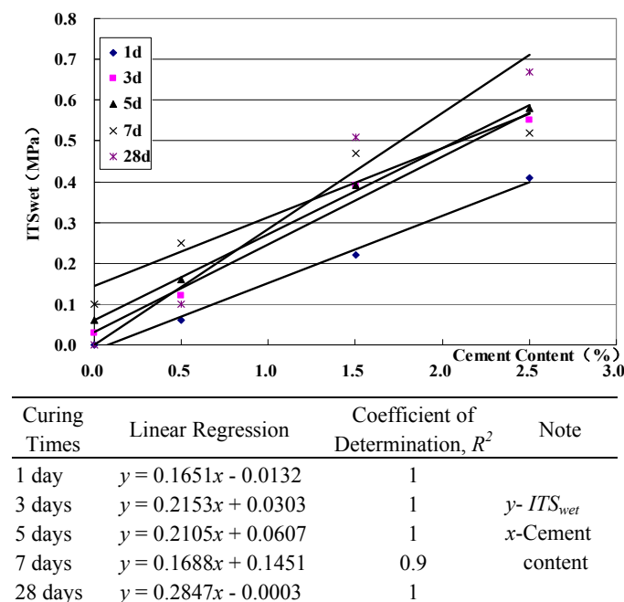
Fig. 7. Relationship Between ITS_{wet} and Cement Content.
