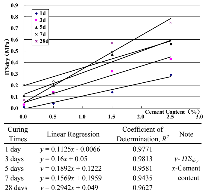
Fig. 6. Relationship Between ITS_{dry} and Cement Content.
