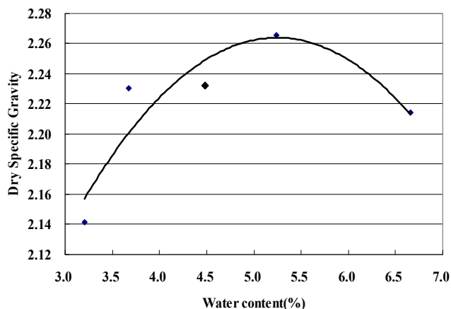
Fig. 1. Relationships Between Dry Specific Gravity and Water Content.
