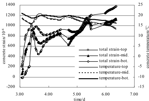
Fig. 6. Concrete Total Strains and Temperatures at Induced Crack III after Cracking.
