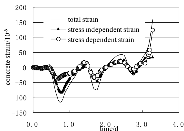
Fig. 12. Concrete Strain Variations at Location a(1).
