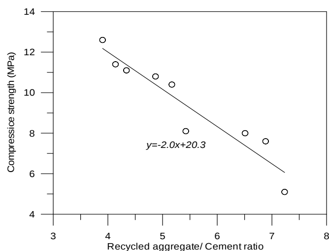
Fig. 4. Relationship between Recycled Aggregate/Cement Ratio and Compressive Strength.
