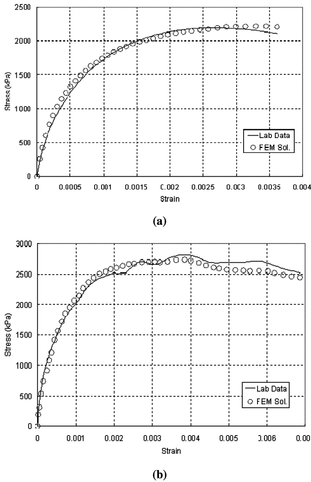
Fig. 4. Stress Prediction Compared to Measured Stress in Lab Tests: (a) 0.000012/sec Reduced Strain Rate; and (b) 0.000026/sec Reduced Strain Rate.
