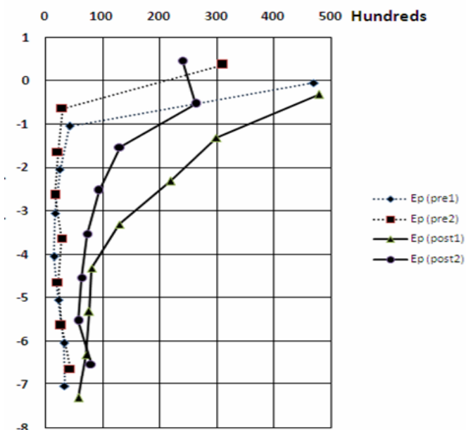
Fig. 5. Menard Modulus Before and After Dynamic Compaction.
