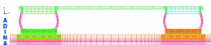
Fig. 8. Contact Surfaces between Tire and Pavement Surface.
