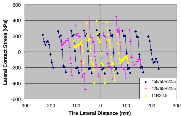
Fig. 18. Comparisons of Lateral Contact Stress among Different Tires.
