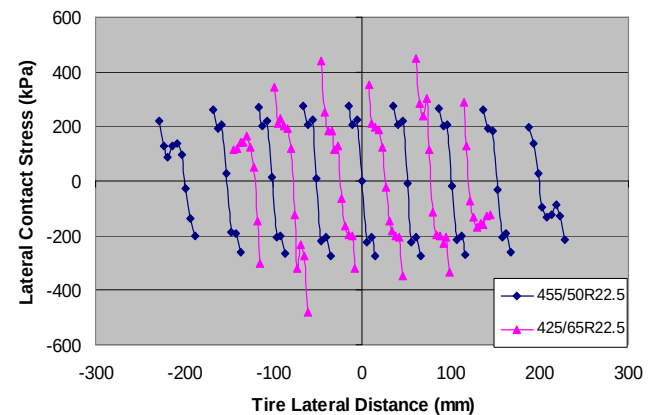
Fig. 16. Predicted Transverse Contact Stress for Wide-base Tires.
