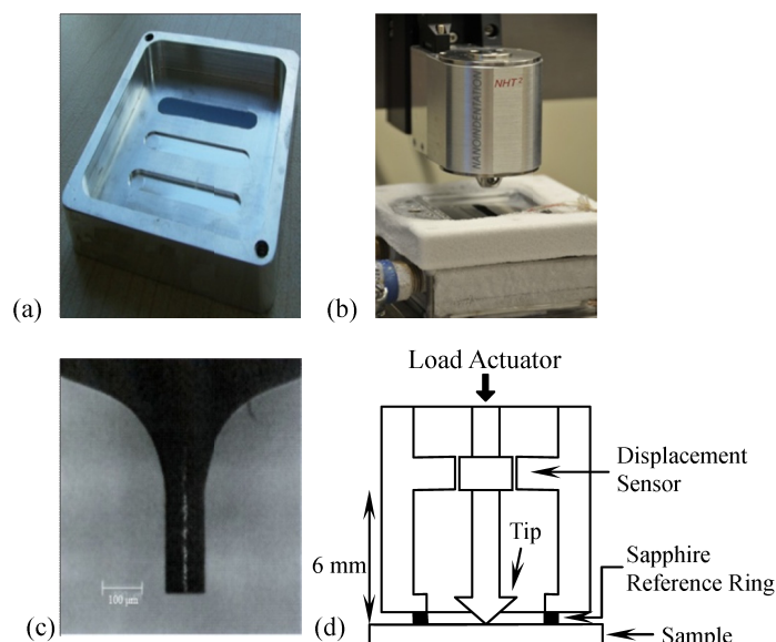
Fig. 1. (a) Sample tray with the 200 micron trough filled with asphalt; (b) Indenter module positioned above the frosted cold stage; (c) Optical image of the 100 micron flat-ended punch; and (d) Schematic of the internal configuration of the CSM NHT 2 indenter head.
