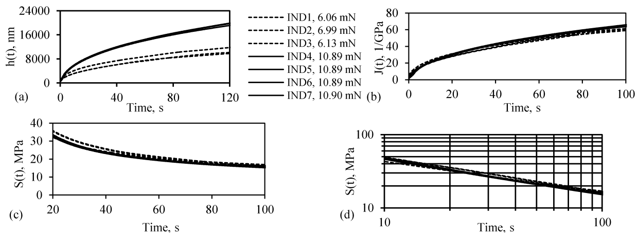
Fig. 2. Typical indentation creep results obtained from a 200 micron thin asphalt cement film at -14^{\circ}\text{C} : (a) Raw data at different creep loads; (b) Compliance versus time at different creep loads; (c) Stiffness versus time at different creep loads; and (d) Creep stiffness master curve (i.e., log-log plot of Fig.2(c)).
