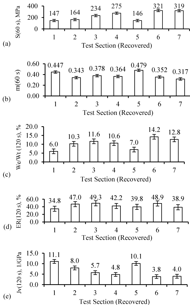
Fig. 3. Indentation creep and recovery data: (a) Creep stiffness; (b) Slope of the creep stiffness master curve (m-value); (c) Elastic versus total work of indentation; (d) Elastic recovery; and (e) Viscous compliance. Note: All tests were done at -14°C and error bars represent \pm 1 pooled standard deviation.
