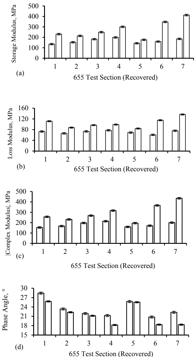
Fig. 5. Dynamic rheological data for recovered binders at 0.5 Hz and -8°C (first column) and -14°C (second column): (a) Storage moduli; (b) Loss moduli; (c) Complex moduli; and (d) Phase angles. Note: Error bars reflect \pm 1 pooled standard deviation.
