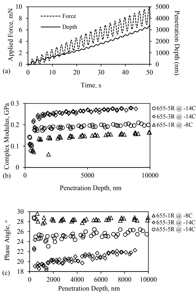
Fig. 4. Typical dynamic indentation results: (a) Raw force and displacement traces; (b) Complex moduli as a function of indentation depth; and (c) Phase angles as a function of indentation depth. Note: (a) shows a single test result obtained on a 400 micron film while (b) and (c) show four replicates each for three different recovered asphalt cements.
