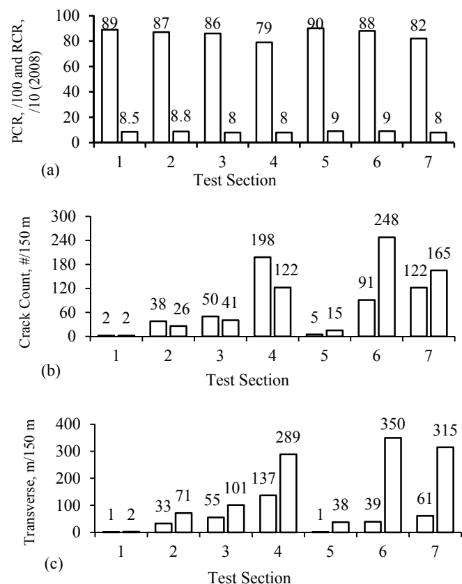
Fig. 7. Pavement distress indicators: (a) Pavement condition rating (PCR) and Ride comfort rating (RCR) indices for August 2008 [6]; (b) Approximate transverse crack counts for 2008 (first column) [6] and 2010 (second column); and (c) Approximate transverse crack lengths for 2008 (first column) [6] and 2010 (second column).
