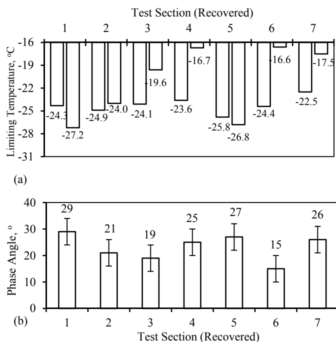
Fig. 6. Conventional grading of asphalt cements recovered from 2009 core samples: (a) BBR and (b) DSR at -14^{\circ}\text{C} . Note: Limiting stiffness temperatures are provided in the first column and limiting m-value temperatures in the second column. Error bars on phase angles provide \pm 1 pooled standard deviation. Significant errors in DSR data show that at this temperature the machine is at the limit of its capabilities with 8 mm parallel plates.
