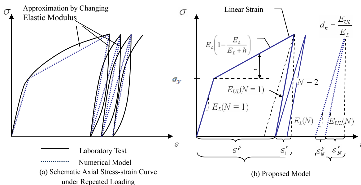
Fig. 1. Schematic Diagram of the Proposed Permanent Deformation Model.
