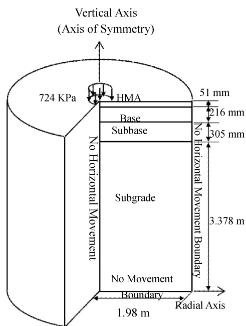
(a) Axisymmetric finite-element model and boundaries
