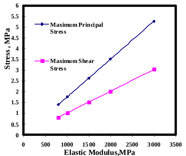
Fig. 3. Stress of BDP with Different Moduli at 60°C
