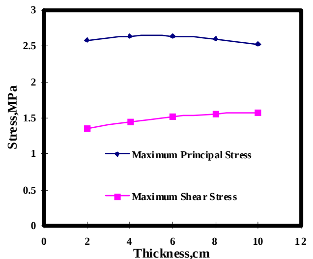
Fig. 5. Stress of BDP with Different Thickness at 60°C.
