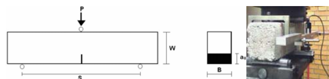
Fig. 7. Arrangement for Fracture Tests with RCC Specimens.
