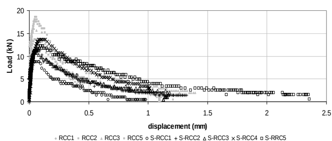
Fig. 9. Superimposition of the Load Versus Displacement Curve for the RCC with Industrial Sand and with Slag (Cement Content of 100 kg/m 3 ).
