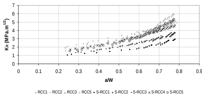
Fig. 11. K_R -curves for RCC (Cement Content of 100 kg/m 3 ) in Terms of Stress Intensity Factor as a Function of the Normalized Crack Length.
