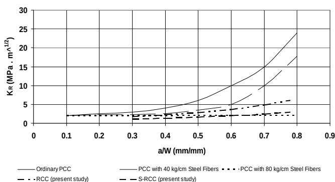
Fig. 14. K_R -curves Obtained from the High-strength Concrete Shown in Fig. 13, of the same Concrete with the Addition of 40 kg/m 3 and 80 kg/m 3 of Steel Fiber (Adapted from Ferreira [6]).
