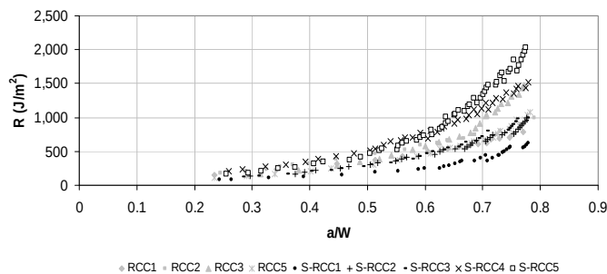
Fig. 10. Superimposition of the R -curves for the RCC with Industrial Sand and with Slag (Cement Content of 100 kg/m 3 ) as a Function of the Normalized Crack Length.
