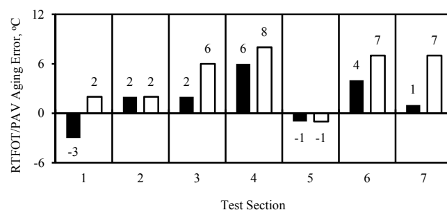
Fig. 6. Approximate RTFO/PAV Aging Errors for 2008 (First Column) and 2009 (Second Column). Note: Grading errors were determined as the difference between the RTFOT/PAV residue grade minus the recovered grade according to AASHTO M320 criteria.
