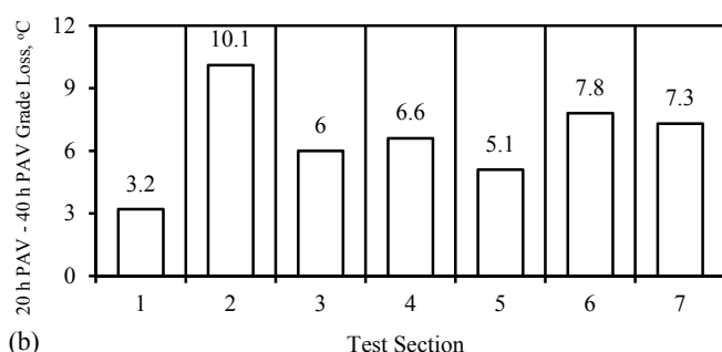
Fig. 10. AASHTO M320 Grades and Grade Losses after 40 hours of PAV Aging Relative to the Standard 20 hours of Aging.
