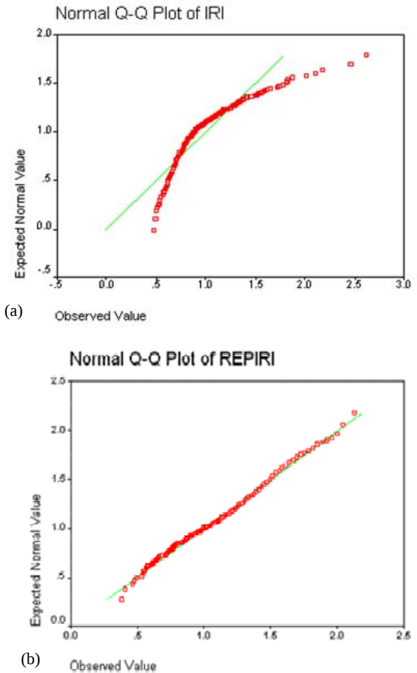
Fig. 2. (a) Q-Q Plot Before Transformation and (b) Q-Q Plot After Transformation.
