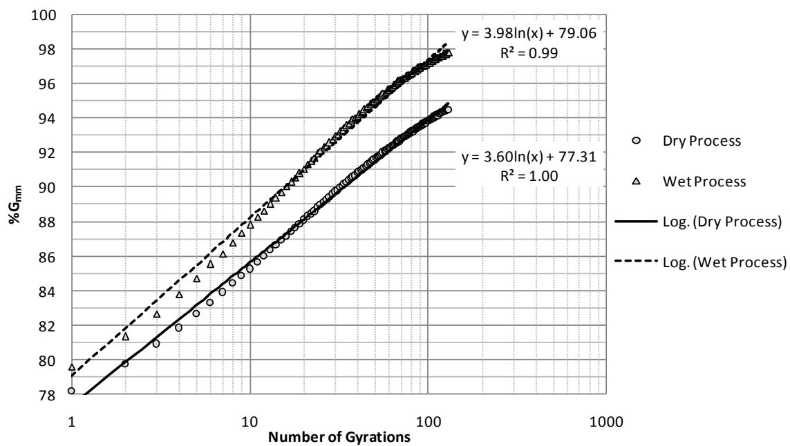
Fig. 4. Gyratory Compaction Curves of the Studied Mixtures.
