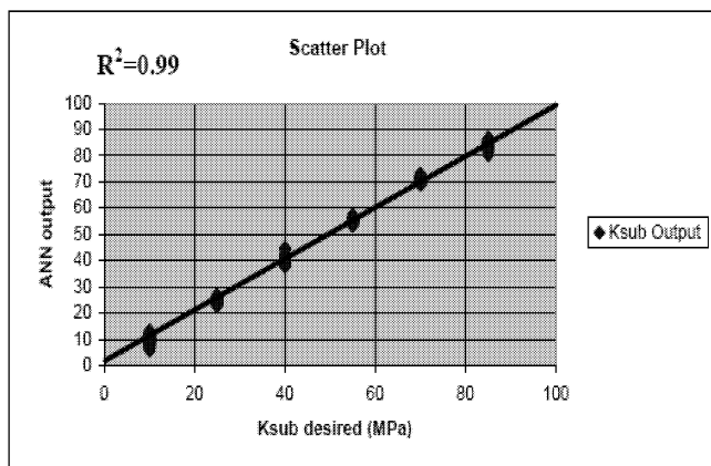
Fig. 7. ANN Prediction of Subgrade Modulus.
