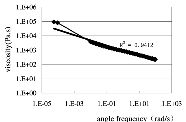
Fig. 5. Viscosity of PG76 from Creep Test and from Frequency Sweep.
