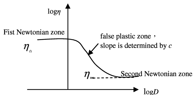
Fig. 2. Curve of Viscosity versus Shear Rate.
