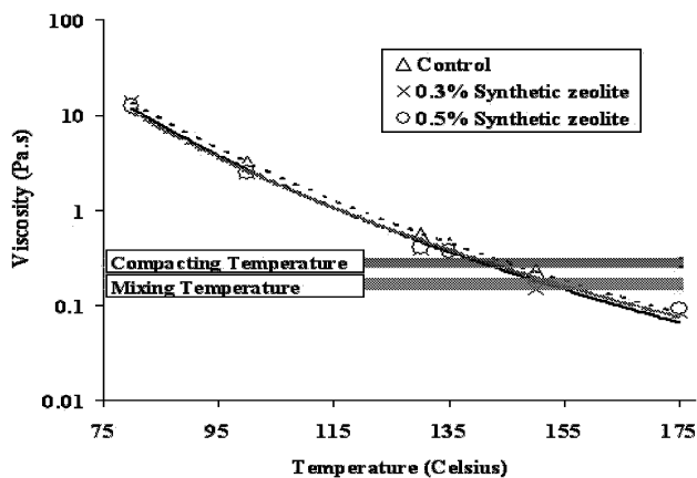
Fig. 3. Comparing Viscosity Test Results of Control and Synthetic zeolite Binder.
