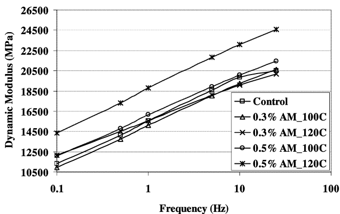
Fig. 5. Dynamic Modulus Test Result at -5^\circ\text{C} .
