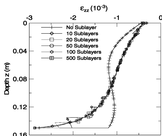
Fig. 8. Vertical Strain ( \epsilon_{zz} ) Variation with Depth in AC Layer.
