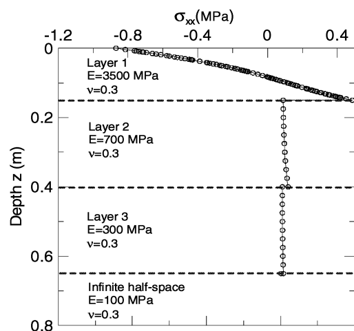
Fig. 2. Horizontal Stress ( \sigma_{xx} ) Jumps at Interfaces in a Flexible Pavement System.
