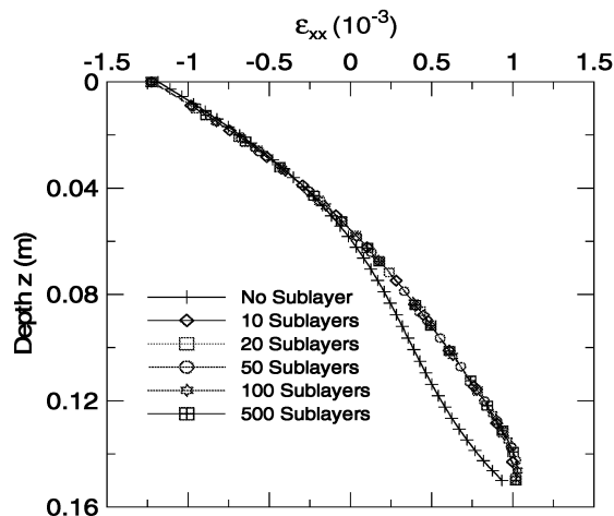
Fig. 9. Horizontal Strain ( \epsilon_{xx} ) Variation with Depth in AC Layer.
