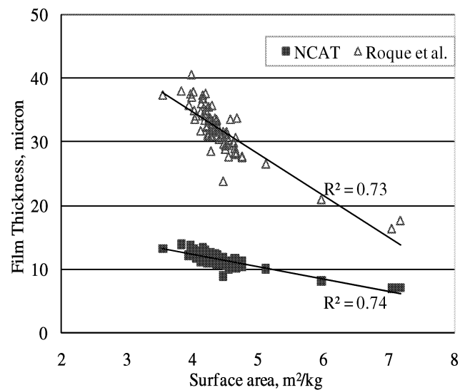
Fig. 2. Asphalt Film Thickness as Related to Surface Area.
