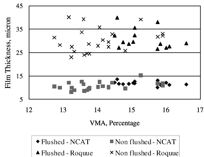
Fig. 6. Asphalt Film Thickness vs. % VMA, Field Cores.
