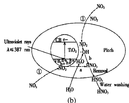
Fig. 2. Photocatalysis and Oxidation Mechanism of Nano-TiO 2 Photocatalyst Immobilized on (a) Concrete and (b) Asphalt.
