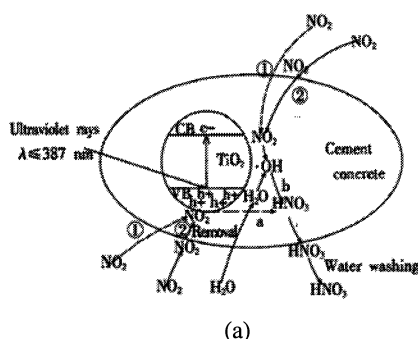
Fig. 2. Photocatalysis and Oxidation Mechanism of Nano-TiO 2 Photocatalyst Immobilized on (a) Concrete and (b) Asphalt.
