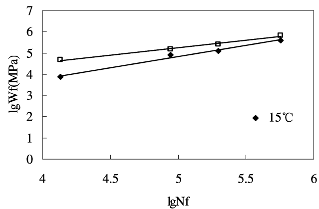
Fig. 7. Beam for Nano-Rubber Modified Asphalt Cycle Time-Strain in Double-Log Coordinate.
