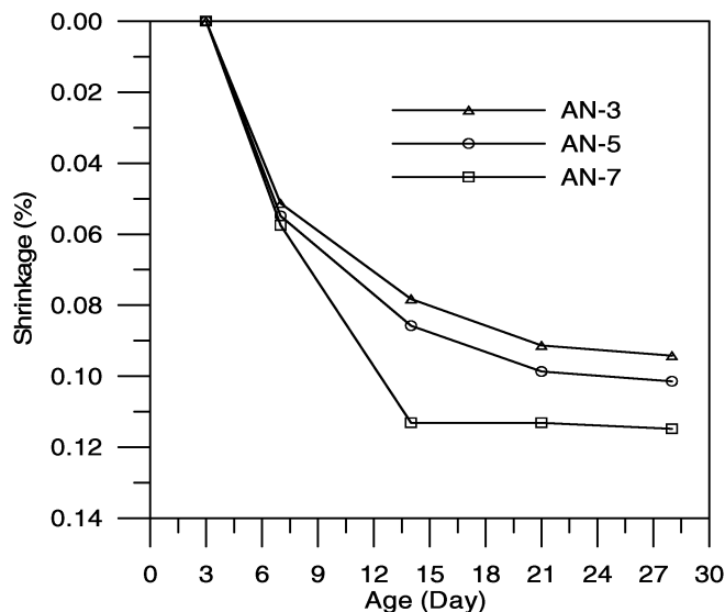
Fig. 4. Shrinkage of CLSM Produced versus Curing Time.
