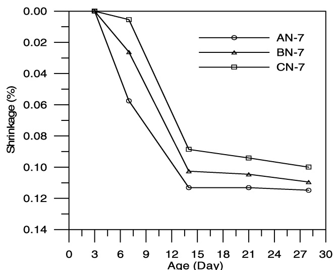
Fig. 5. Shrinkage of CLSM Produced versus Curing Time.
