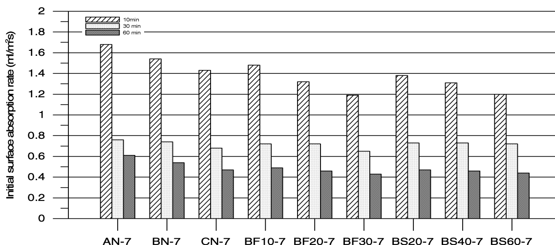
Fig. 8. ISAT Plot for Various CLSM Mixes.
