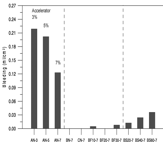
Fig. 3. Bleeding of Various CLSM Mixes.
