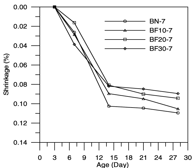
Fig. 6. Shrinkage of CLSM Produced versus Curing Time.
