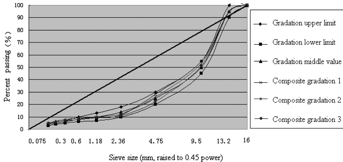
Fig. 1. Three Preliminary Aggregate Gradation Curves.
