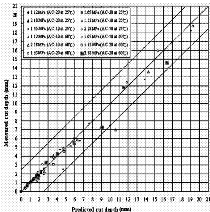
Fig. 6. Measured Versus Predicted Rut Depths.
